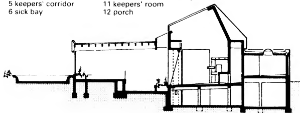
7 Section (6)
